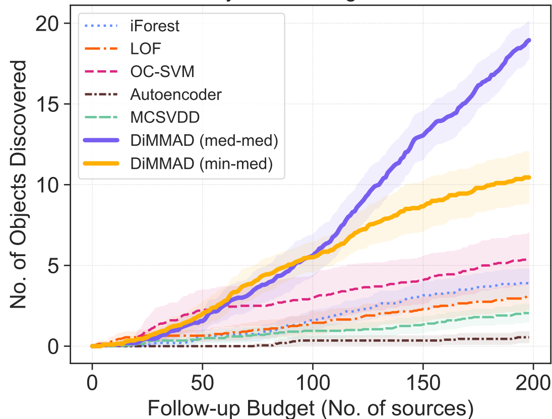
Anomaly: uLens-Single-GenLens
